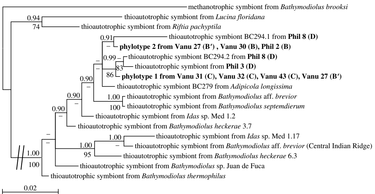
Figure 4. Bayesian tree obtained from the analysis of the 16S rRNA dataset. Sequences obtained in this study are in bold. Substitution model selected from MrAIC: GTR+ [\Gamma] +I. Posterior probabilities (PP) and bootstraps values obtained from ML analysis are given above and below nodes, respectively. PP and bootstraps values lower than 0.90 and 50%, respectively, are not shown. Scale bar represents 2% estimated base substitution. The broken branch represents 13% estimated base substitution.
