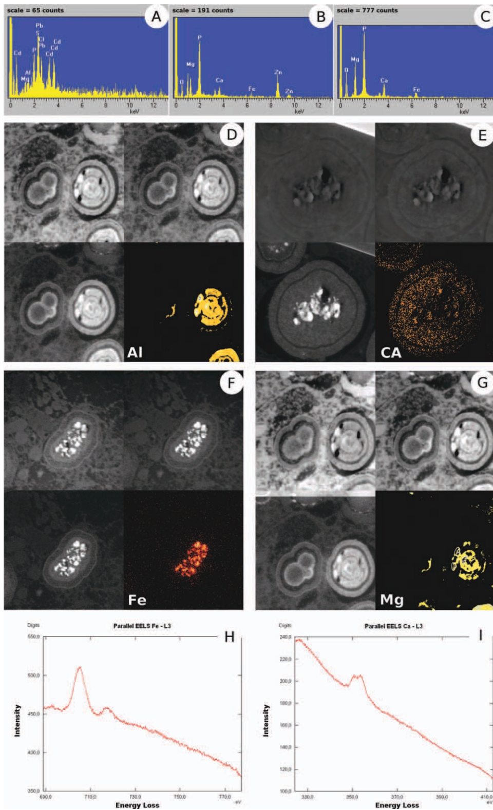
Fig. 2. EDX and EFTEM analyses. (A) EDX spectrum obtained from a pellet contaminated with \text{CdCl}_2 and \text{Pb}(\text{NO}_3)_2 where cadmium and lead peaks are visible. (B, C) Ca, Fe, Mg, P and Zn are detected on EDX spectra obtained from a spherocrystal of S. pugilis (B) and S. gigas (C) not contaminated. Peaks for Al and Mn have also been detected in some others spherocrystals of S. gigas . (D–G). Spherocrystals of uncontaminated S. gigas observed by Electron Spectroscopic Imaging (ESI) using the three windows method. The upper left image is taken just before the element peak, the upper right image corre-
