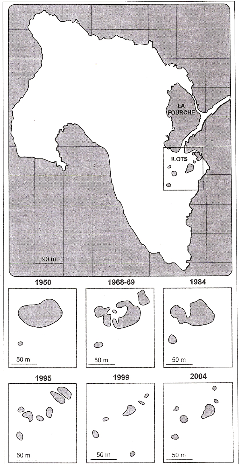
Fig. 4 – Morphological evolution of the small islands between 1950 and 2004.
